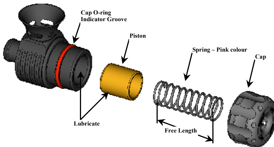
Figure 3 Exploded View of the Kompact SS BOV
